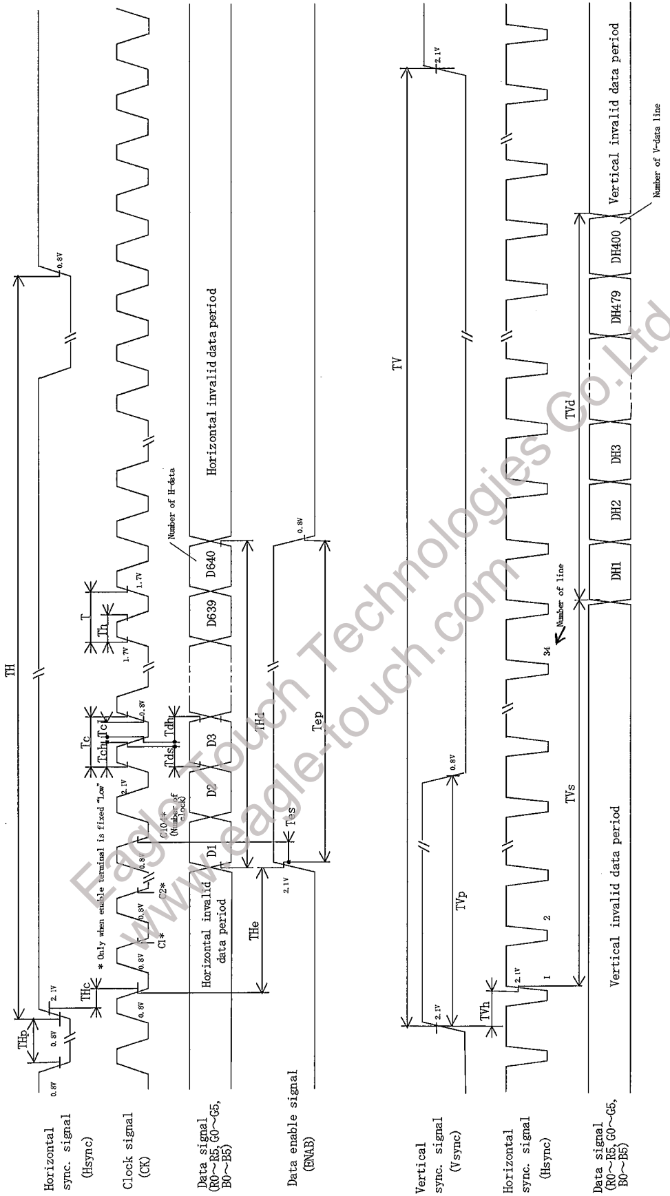
Fig2-2 Input signal waveforms (400 line mode)
