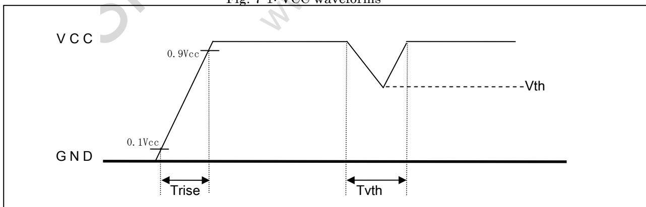
Fig. 7-1: VCC waveforms
