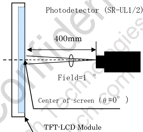
Fig11-2 Luminance / Chromaticity / Contrast measurement method
